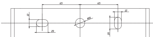
MEGAFOCUS 238x50 mm
