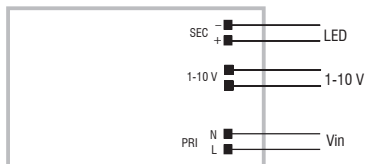
1...10 V diagram - Collegamento 1...10 V
