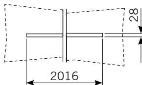
S.2322 Ceiling cut out
