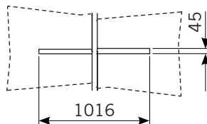
S.2371 Ceiling cut out
