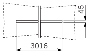
S.2373 Ceiling cut out
