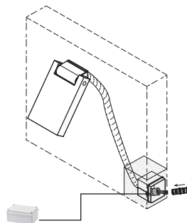
Junction box 120x80x50mm (NOT SUPPLIED) Scatola di derivazione 120x80x50mm (NON FORNITA) Anschlussdose 120x80x50mm (NICHT GELIEFERT) Boutier de raccordement 120x80x50mm (NON FOURNI) Caja de conexiones 120x80x50mm (NO INCLUIDO)
