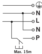
Junction box 120x80x50mm (NOT SUPPLIED) Scatola di derivazione 120x80x50mm (NON FORNITA) Anschlussdose 120x80x50mm (NICHT GELIEFERT) Boutier de raccordement 120x80x50mm (NON FOURNI) Caja de conexiones 120x80x50mm (NO INCLUIDO)
