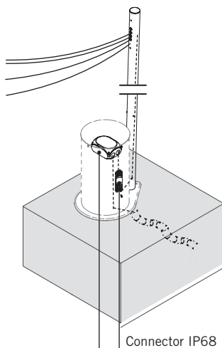
Connector IP68
