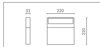
S.7236W LEDs 12,5W - 230V
