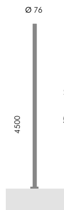
S.2845 Ø 76 mm CYLINDRICAL POLE WITH BASE Pole total height 4500mm Provided with inspection door
