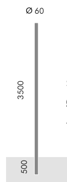
S.2842 Ø 60 mm CYLINDRICAL POLE TO BE BURIED Pole total height 4000mm To be buried for 500mm
