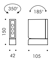
MINIKEEN 3 LED Ø 105
