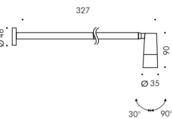
FLOWER Ø35 A BRACCIO L330 Flower Ø35 with arm L330
