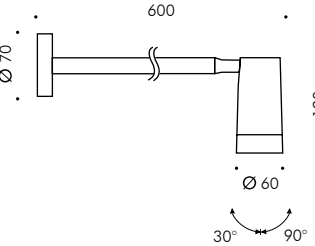
FLOWER ZOOM Ø60 A BRACCIO L600 Flower ZOOM Ø60 with arm L600
