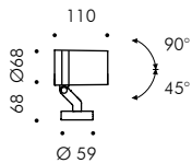
MICROSTAGE Ø68 LAMA DI LUCE Microstage Ø68 blade of light
