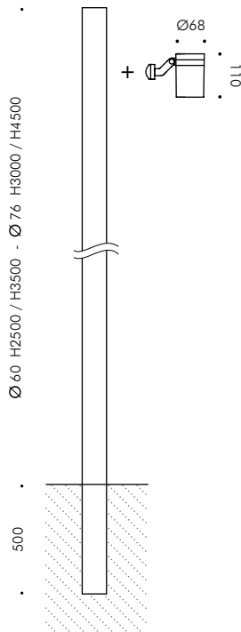
MICROSTAGE Ø68 LAMA DI LUCE ATTACCO A PALO Microstage Ø68 blade of light pole mounted
