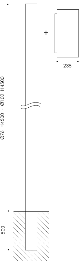
MEGASMOOTH H420 ATTACCO A PALO Megasmooth H420 pole attachment
