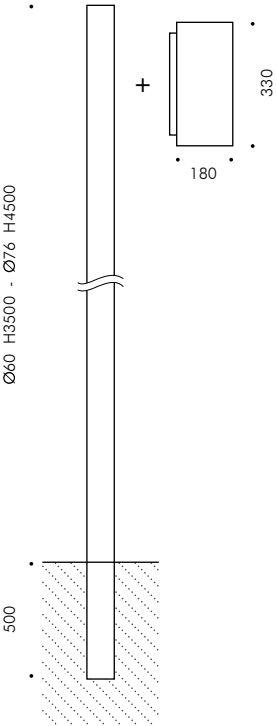
MEGASMOOTH H420 ATTACCO A PALO Megasmooth H420 pole attachment
