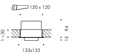
CATCH QUADRATO 4 LED INCASSO \varnothing 130 Catch square 4 LED recessed mounted \varnothing 130
