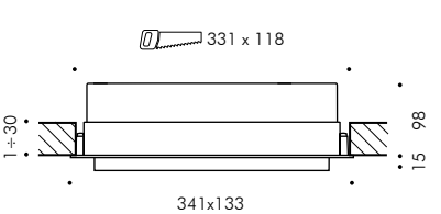
CATCH RETTANGOLARE 20 LED INCASSO L340 Catch rectangular 20 LED recessed mounted L340
