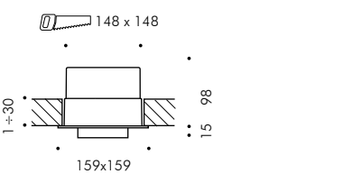
CATCH QUADRATO 9 LED INCASSO \varnothing 160 Catch square 9 LED recessed mounted \varnothing 160
