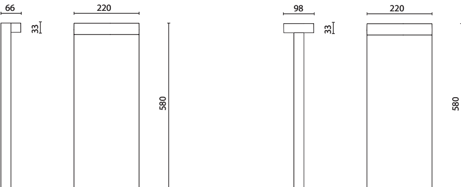
MINI-LOOK L=220mm H=580mm
